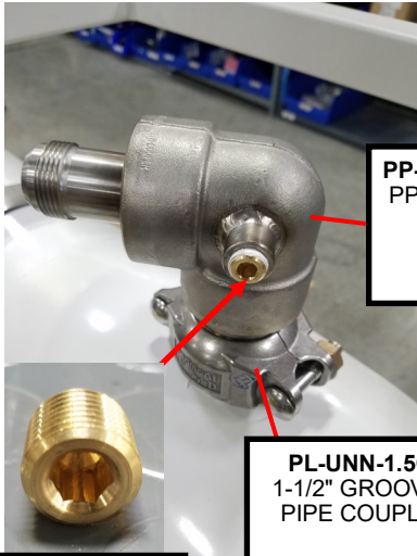
PL-HP-1/4BR 1/4" COUNTER SUNK HEX PLUG (BRASS)
