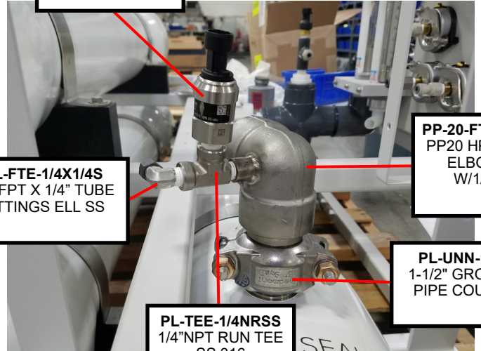
EL-SSR-1500PT1 0-1500 PSI PRESSURE TRANSDUCER SS 1
